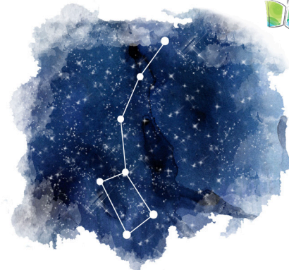
Ursa Minor (Little Dipper)
